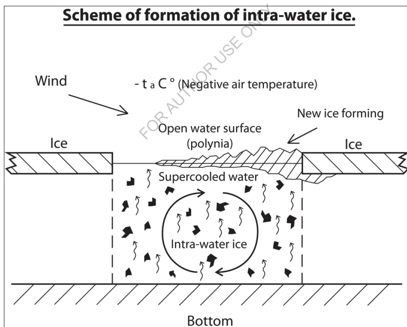
Figure 1. Frazil ice formation in supercooled water under effect of wind chill due to wind and negative air temperature.
