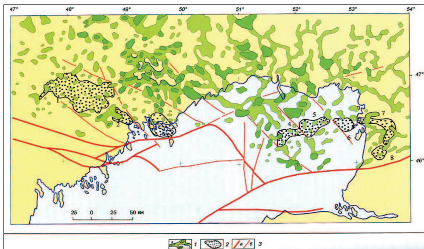
Figure 4. The diagram of salt tectonics and adjacent dry land in the North Caspian (according to drilling, seismic survey and gravimetric data) [11]
