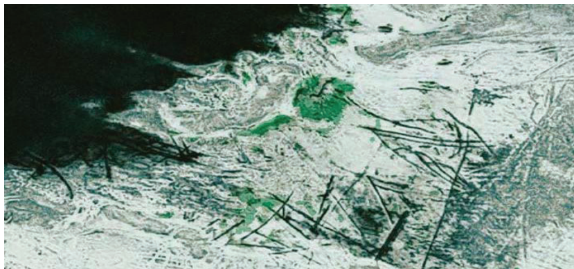
Figure 3. Gouges of ice exaration in satellite image of the Aral sea coast, the scale of the image - 4x6 km (Scanex).
