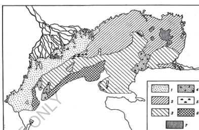
Figure 3. The ice condition status as of February 3, 1984 by the AES data.
