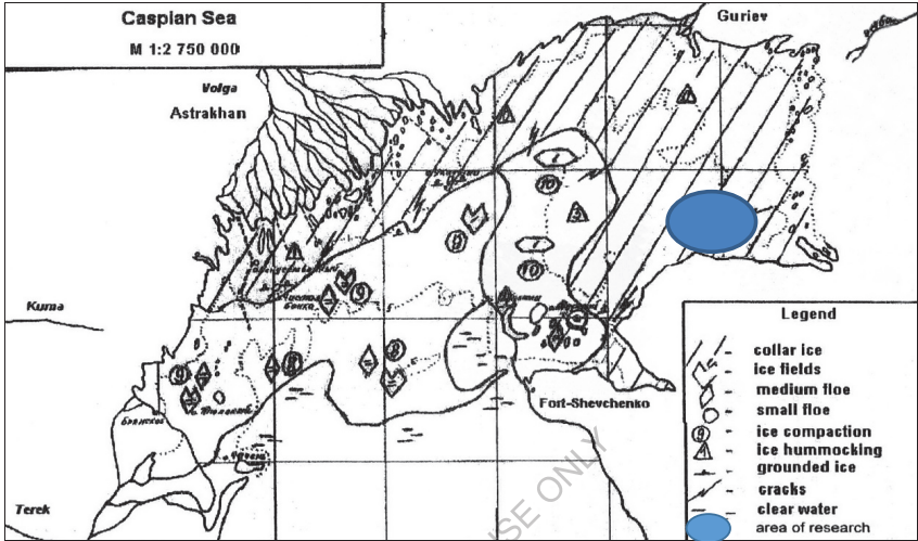
Figure 2. Ice cover in the Northern Caspian on February 6, 1997.
