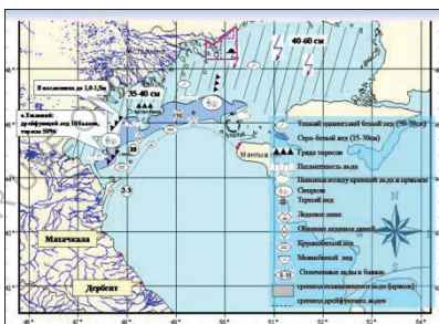
Figure 2. Ice status as per 30 of January 2008.
