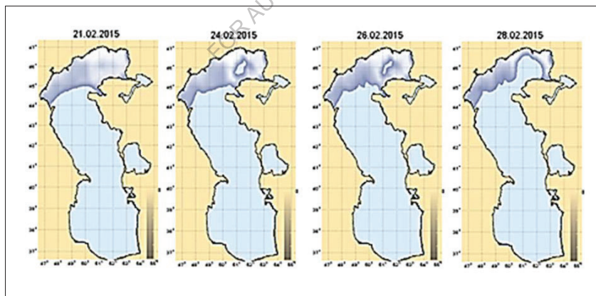
Figure 5. Diagram of the salt domes and polynyas in the North Caspian.
