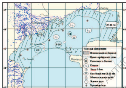
Figure 1. Ice status as per 29 of December 2007.
