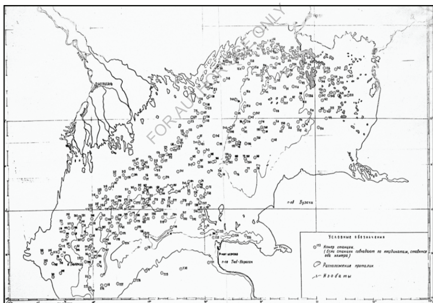
Figure 3. The diagram of salt tectonics and adjacent dry land in the North Caspian (Brusilovsky, 1978).
