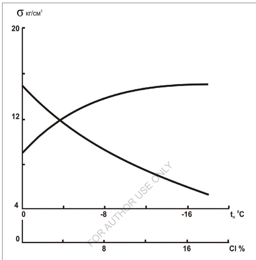
Figure 7. Smoothed ice strength values in the North Caspian related to its temperature and chlorinity (salinity).
