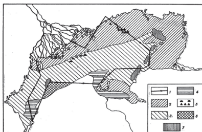
Figure 2. The ice condition status as of January 30, 1984 by the avia survey data.
