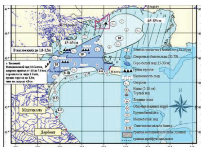
Figure 3. Map of factual ice edge location and ice characteristics as per 21 of February 2008.
