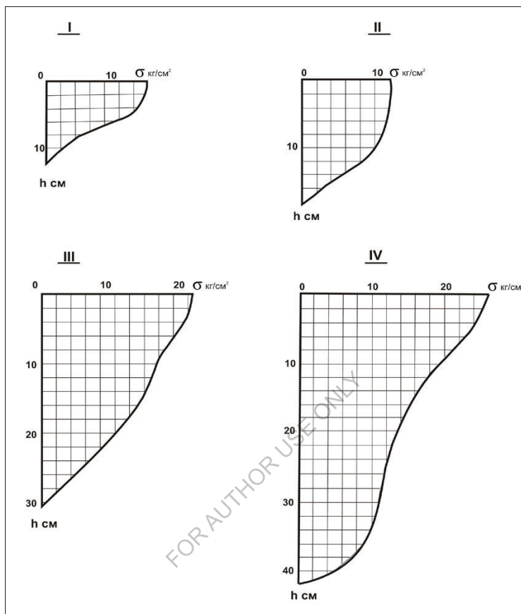
Figure 8. The curves of the ice strength at points located in the eastern part of the North Caspian:
